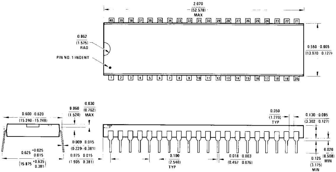
Plastic Dual-In-Line Package (N) Order Number INS1771N-1
